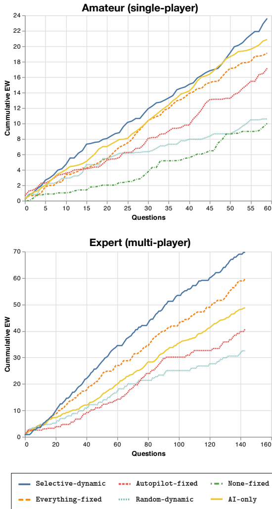
Figure 2: Mean cumulative EW score under each condition by amateurs (top) and experts (bottom). The selective condition performs the best amongst all human-AI cooperative settings.
